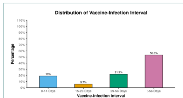
Figure 6. Association of cases with post-vaccine duration
